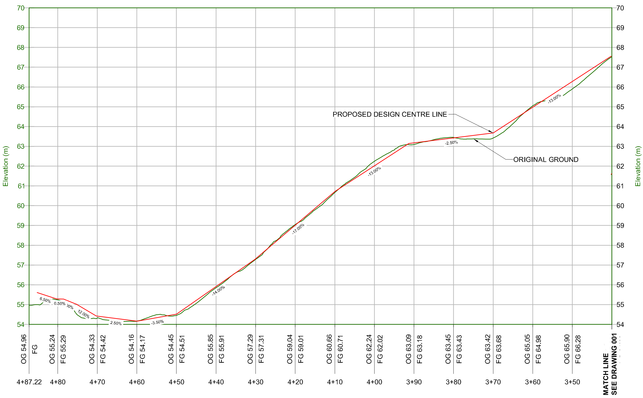
4 TRAIL - PROFILE VIEW 001 HORIZONTAL 1:500 VERTICAL 1:100
