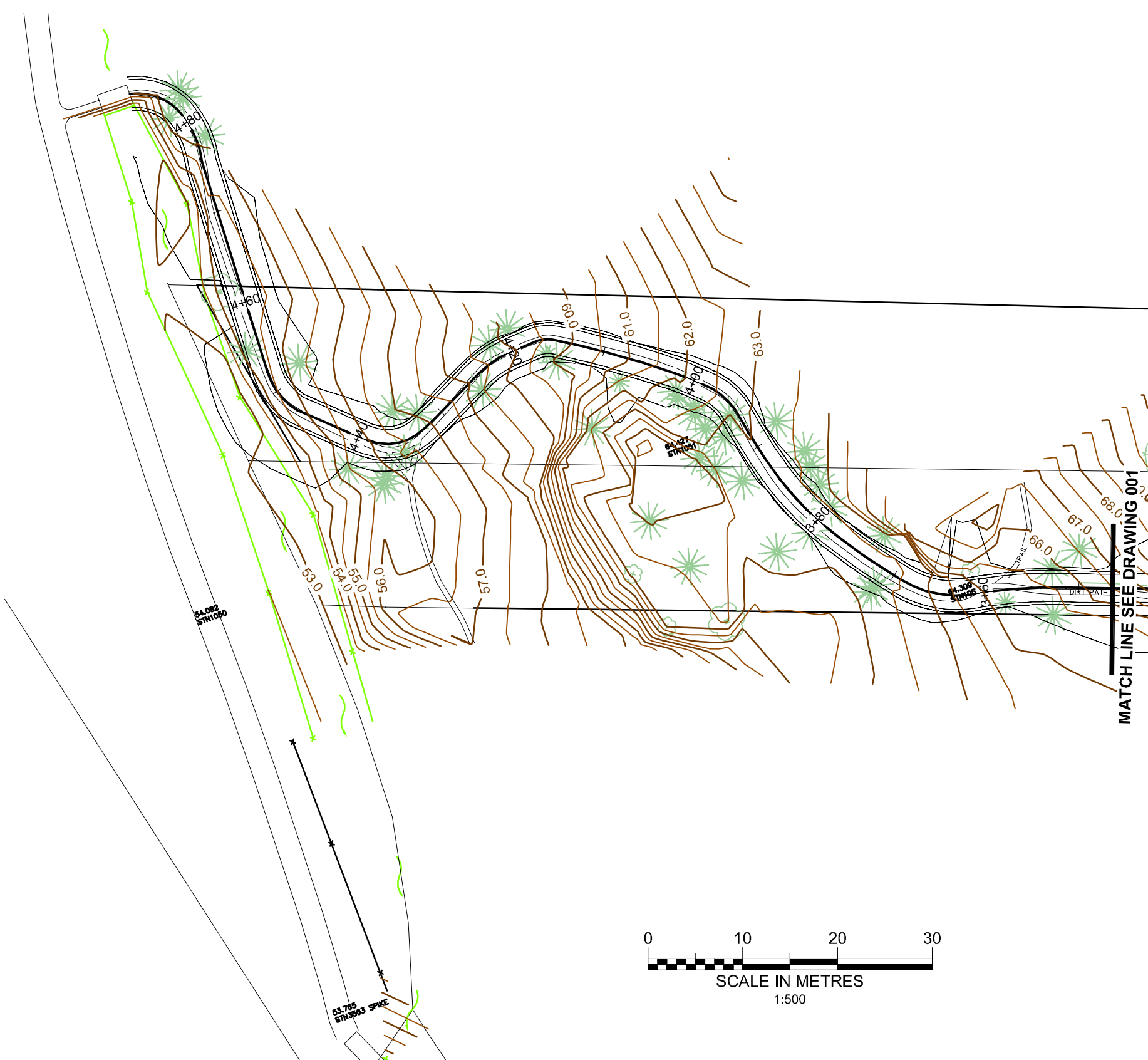
3 TRAIL - PLAN VIEW 001 1:500
